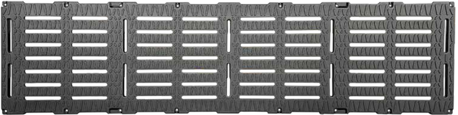
AGRI-8008 Floor Specifications: 8' L x 2' W x 1.625" H / 244 cm L x 61 cm W x 4 cm H Weight: 28 lbs. / 12.7 kg
